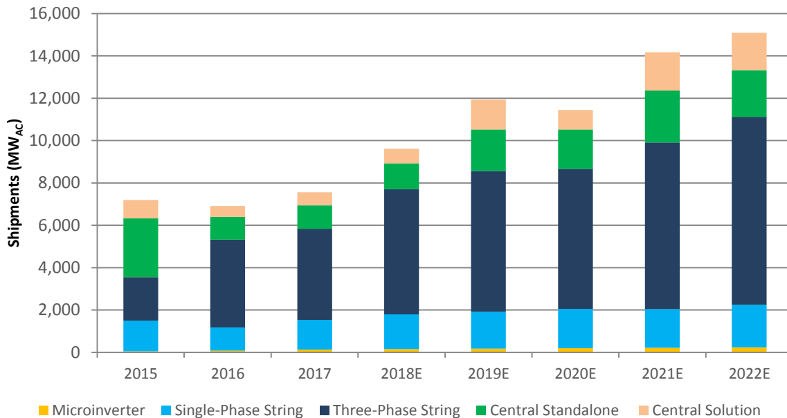
Figure 5 EU inverter shipments by technology (MWac) E=Estimate
