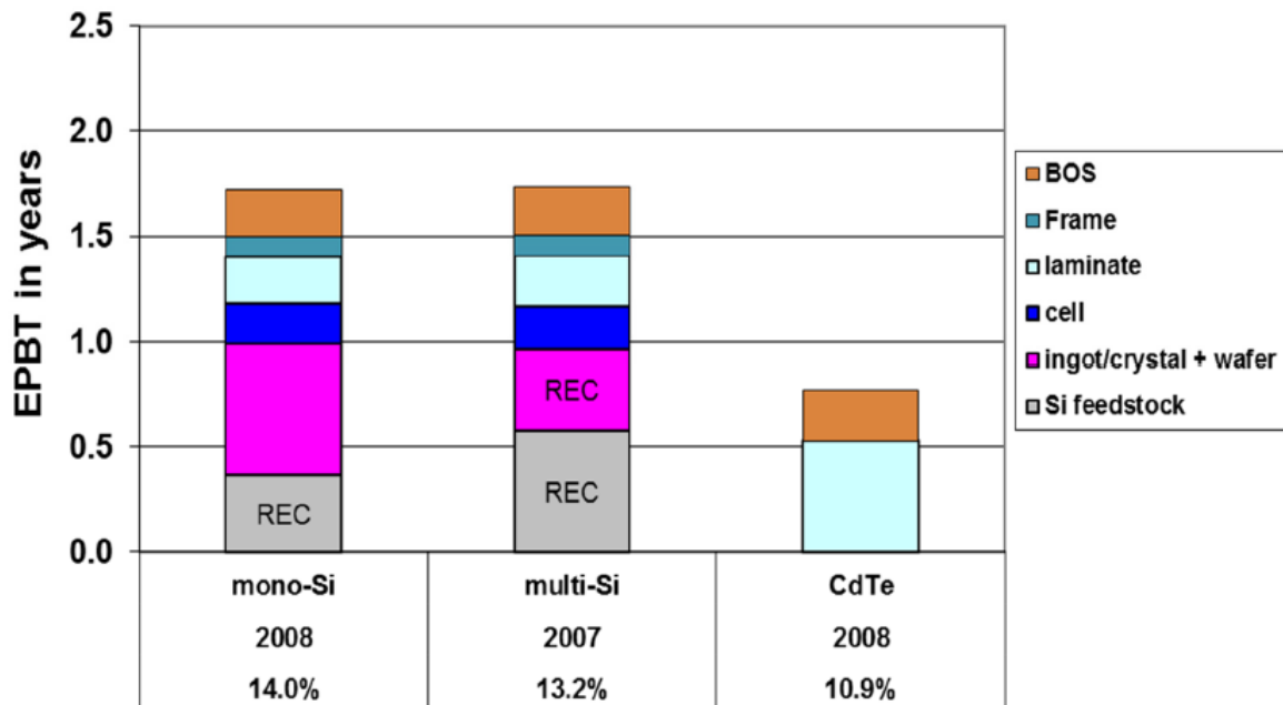
Figure 14: (taken from Frischknecht et al. 2015) Energy payback time (EPBT) of rooftop mounted PV systems for European production and installation under Southern European irradiation of 1700 kWh/m 2 /yr and performance ratio of 0.75. Data adapted from de Wild Scholten (2009) and Fthenakis et al. (2009). They were harmonized for system boundary and performance ratios, according to IEA Task 12 LCA Methodology Guidelines. REC corresponds to REC product-specific Si production; the corresponding LCI data are not publicly available.
