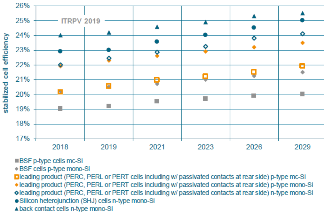
Figure 7. Average stabilised efficiency level for C-Si solar cells (156 x 156mm 2 )
