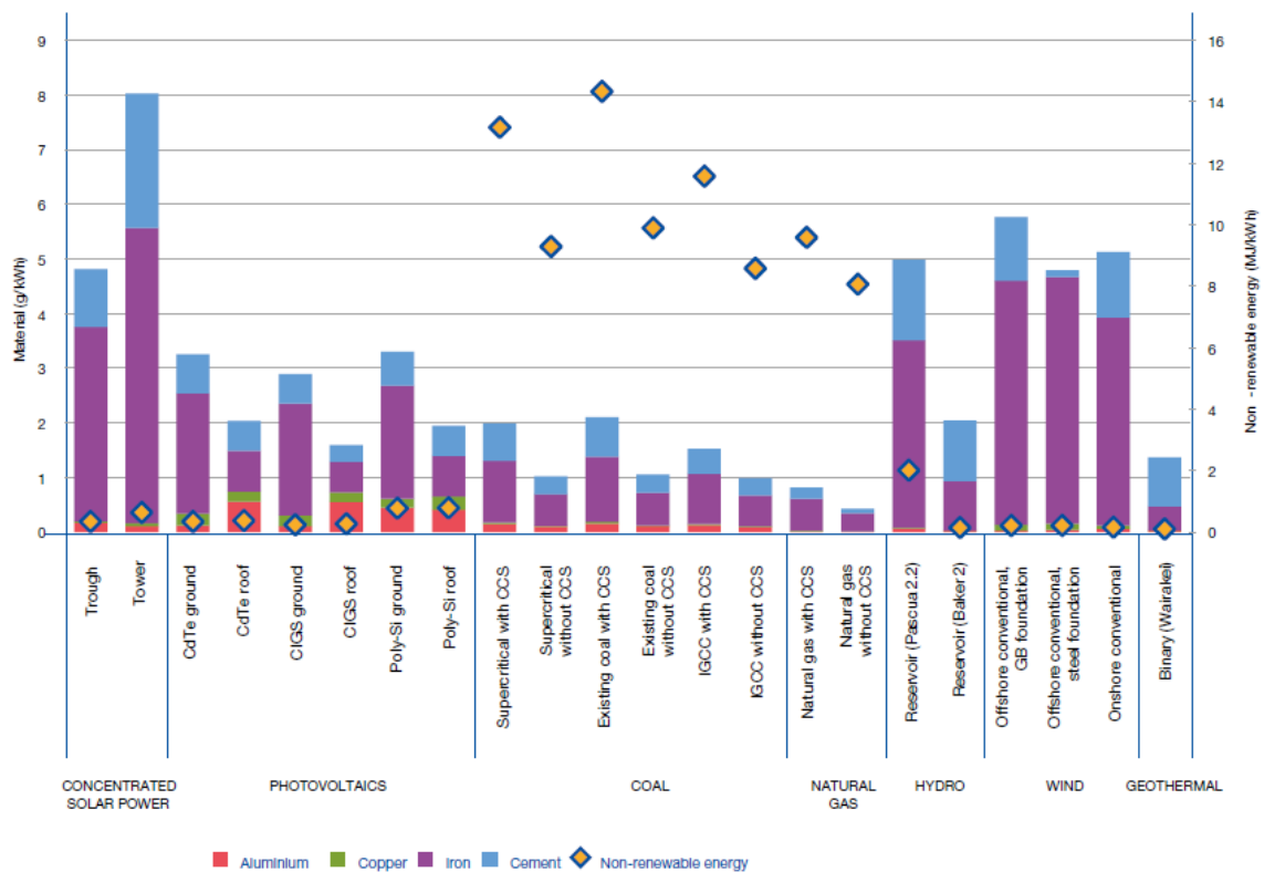
Figure 18: (taken from UNEP 2016) Bulk material and non-renewable energy requirements per unit power produced.
