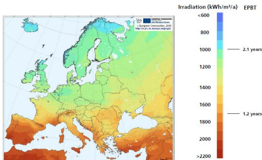
Figure 12. Map of European solar irradiation and indicative Energy Payback Times (EPBT)
