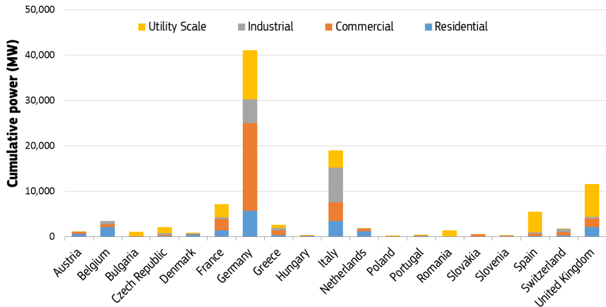
Figure 6. Cumulative Capacity installed in most European countries up to 2016 in MW DC .
