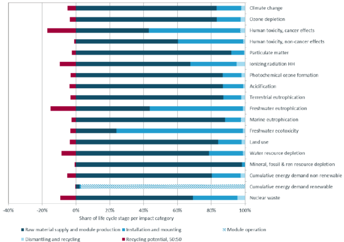
Figure 13 (taken from Wyss et al., 2015): Environmental impact results (characterized, indexed to 100 %) of 1 kWh of DC electricity produced with a residential scale (3 kWp) PV system with average PV modules mounted on a slanted roof. The potential benefits due to recycling are illustrated relative to the overall environmental impacts from production to end-of-life.
