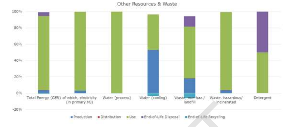
Figure 5.4: Contribution of different life cycle phases to other resources and waste of a professional high pressure cleaner
