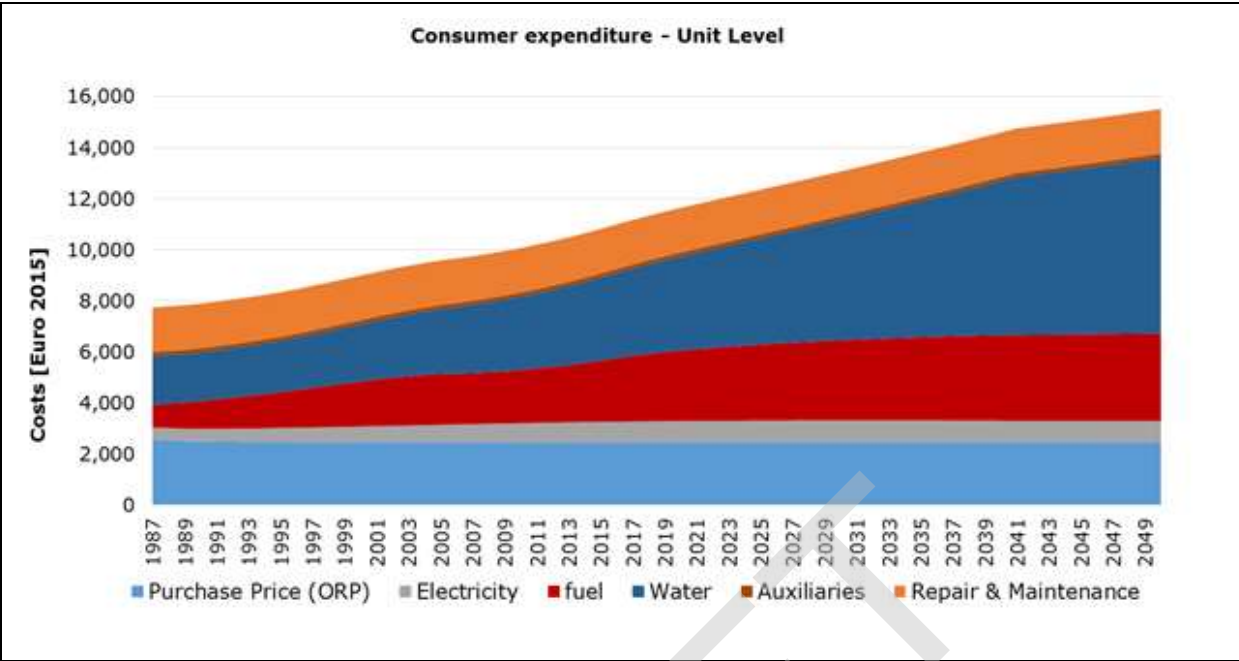
Figure 5.14: Life cycle costs per unit for BC5 (in 2015 EUR equivalent).
