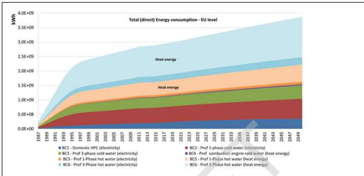
Figure 5.18: Total direct energy consumption for each base case for EU-28. Energy consumption for hot water HPCs is presented separately for electric and heat energy.
