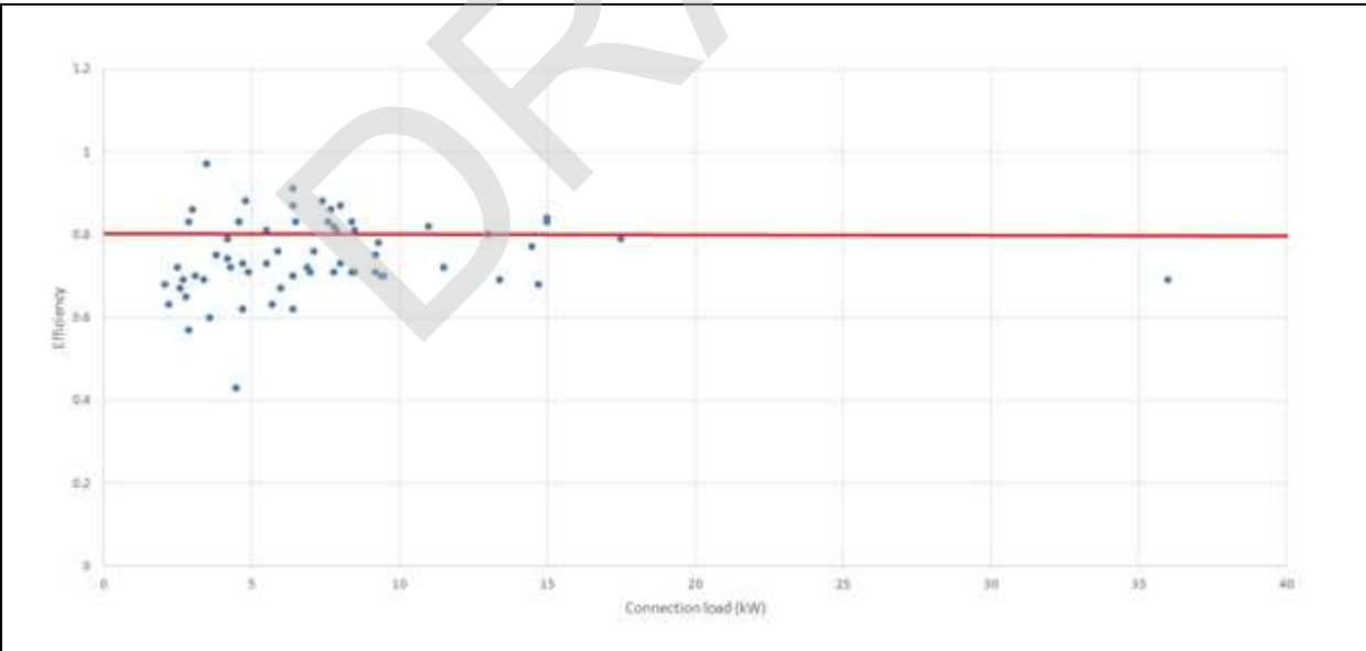
Figure 7.3: Threshold proxy efficiency level for professional HPCs 3 phases. Total number of datapoints is 67.
