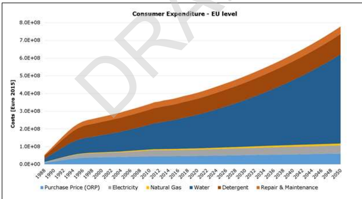
Figure 5.11: Life cycle costs at EU level for BC3 (in 2015 EUR equivalent).
