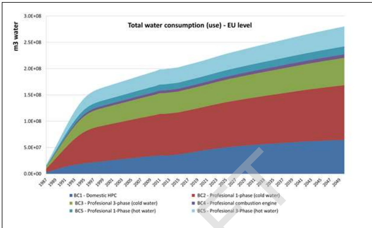
Figure 5.19: Total water consumption for each base case for EU-28.
