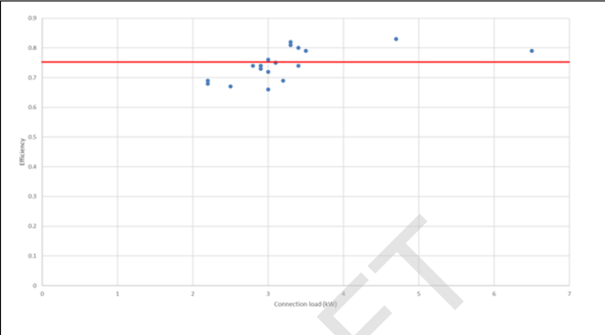
Figure 7.2: Threshold proxy efficiency level for professional HPCs 1 phase. Total number of datapoints is 20.
