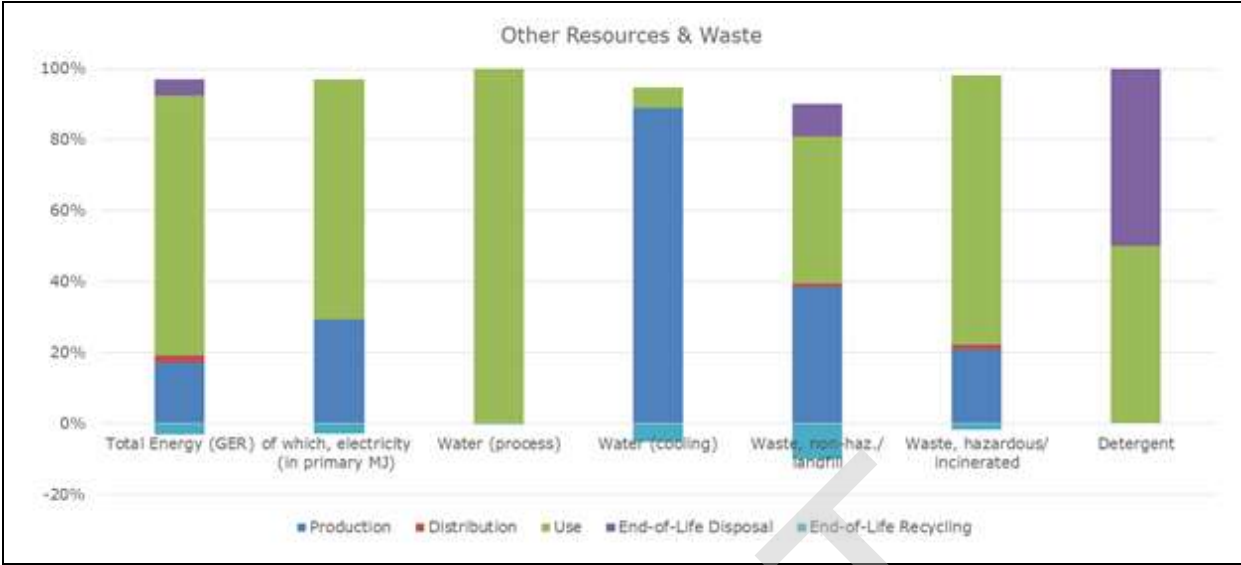
Figure 5.1: Contribution of different life cycle phases to other resources and waste of a domestic high pressure cleaner
