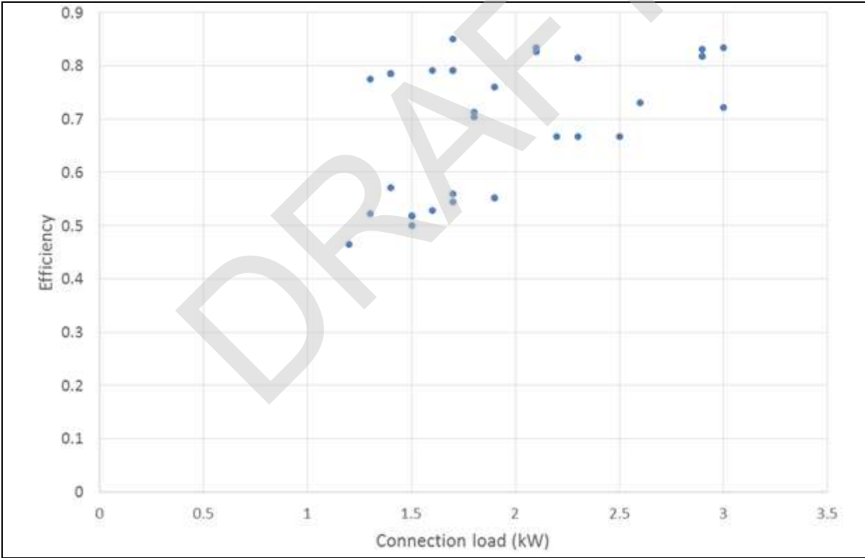
Figure 6.2: Proxy efficiency level for professional HPCs 1 phase.
