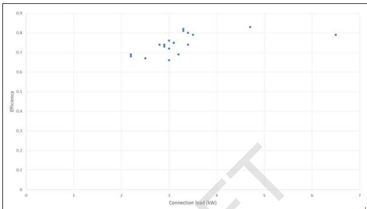
Figure 6.3: Proxy efficiency level for professional HPCs 3 phases
