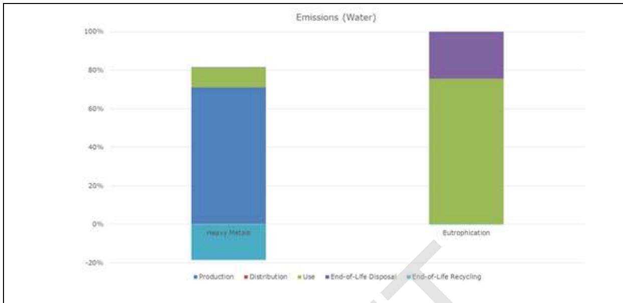
Figure 5.3: Contribution of different life cycle phases to emissions to water of a domestic high pressure cleaner
