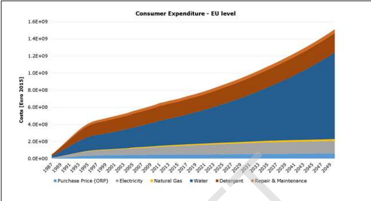
Figure 5.9: Life cycle costs at EU level for BC2 (in 2015 EUR equivalent).
