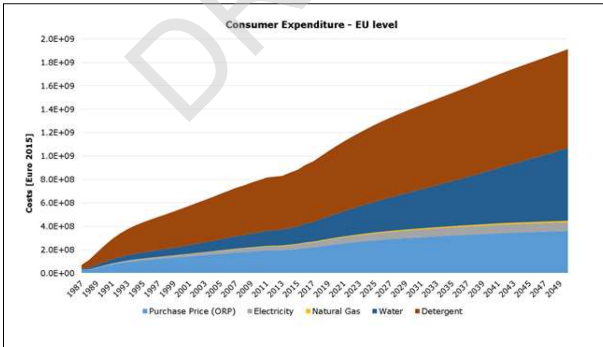
Figure 5.7: Life cycle costs at EU level for BC1 (in 2015 EUR equivalent).
