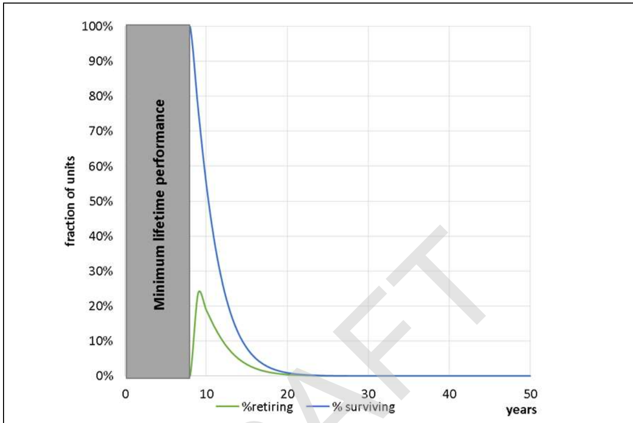
Figure 7.5: The new Weibull lifetime distribution for domestic HPC due to the reparability and durability requirements.
