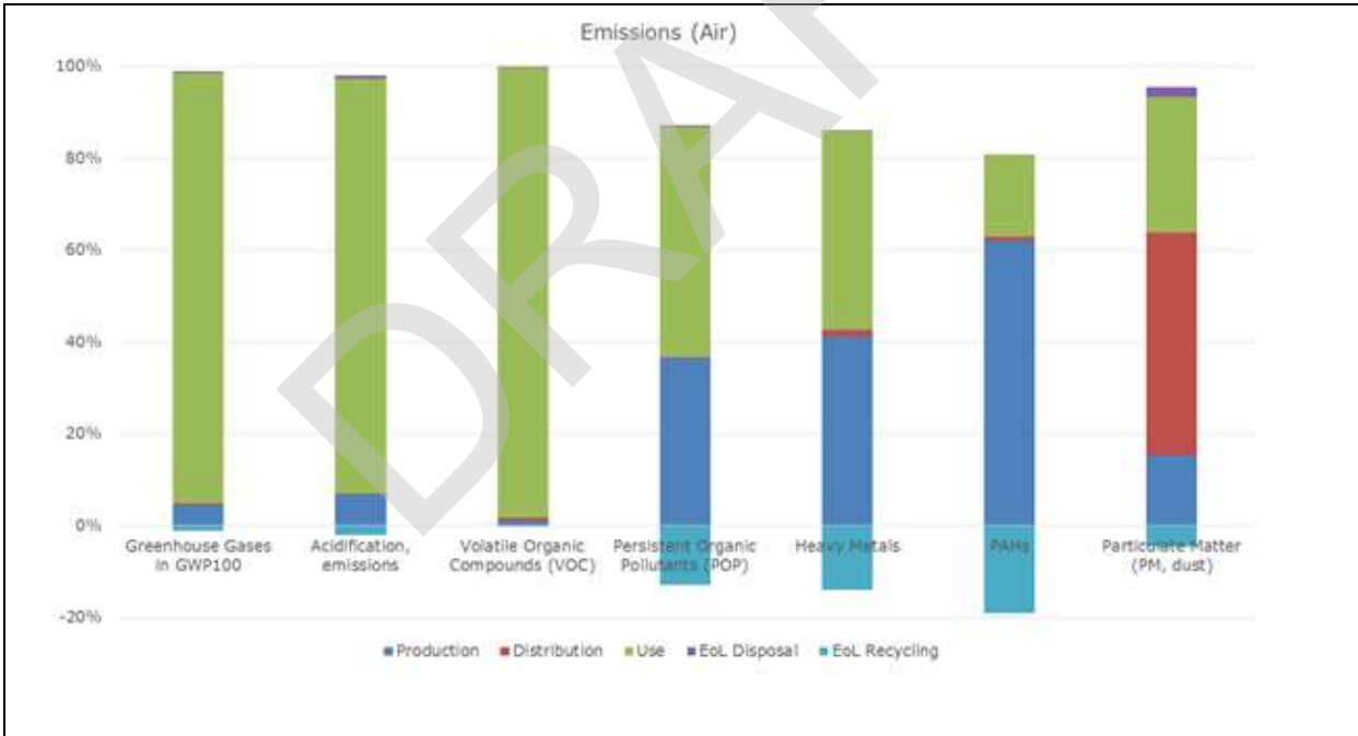
Figure 5.5: Contribution of different life cycle phases to emissions to air of a professional high pressure cleaner
