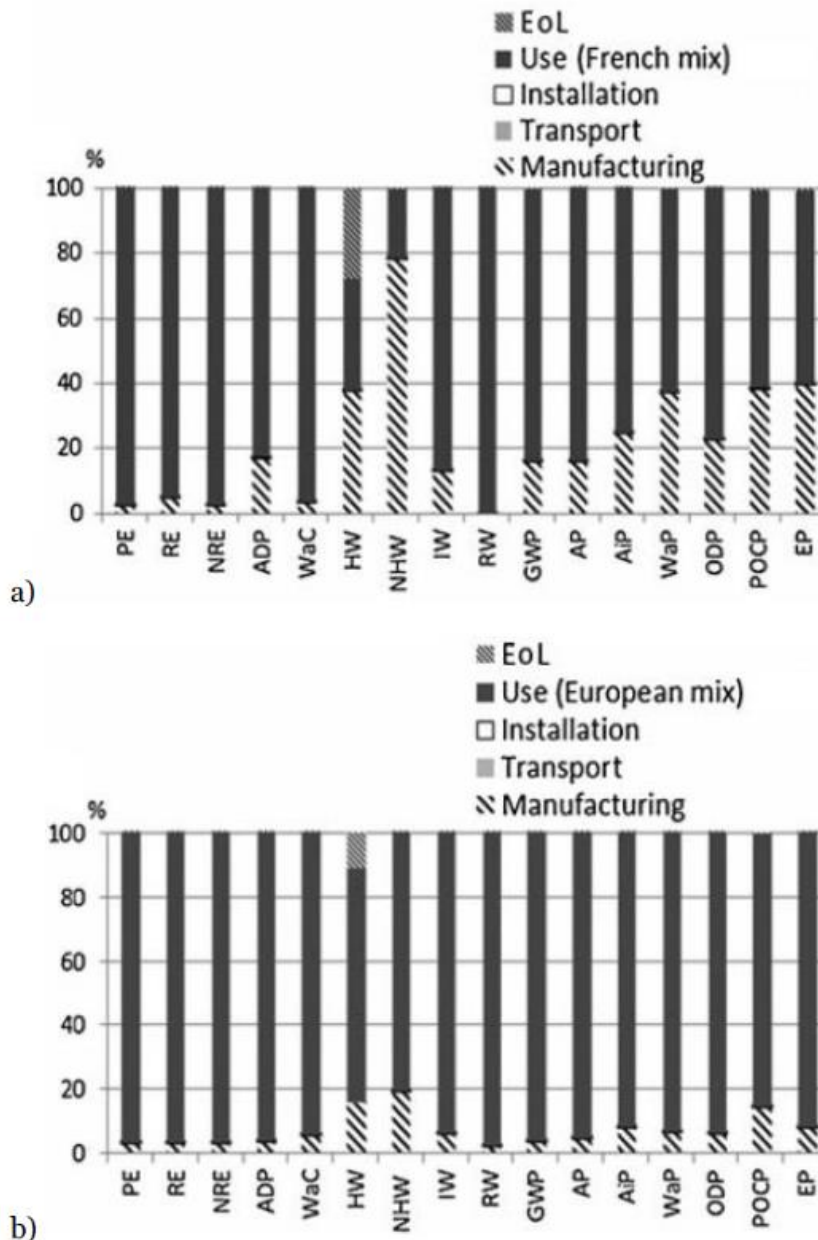
Figure 3-5 Division of environmental impacts of a LED downlight luminaire into life cycle stages with the energy consumption modelled with a) an average French electricity mix and b) an average European electricity mix. Adapted from (Tähkämö et al., 2013).
