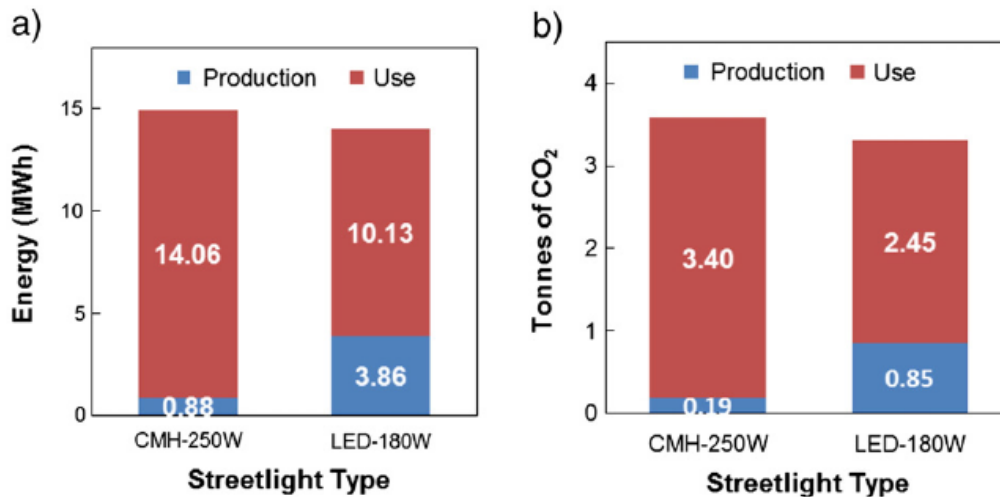
Figure 3-6 (a) Energy consumption and (b) carbon dioxide emissions during production and use phase for CMH and LED streetlights (Hadi, S. et al., 2013)
