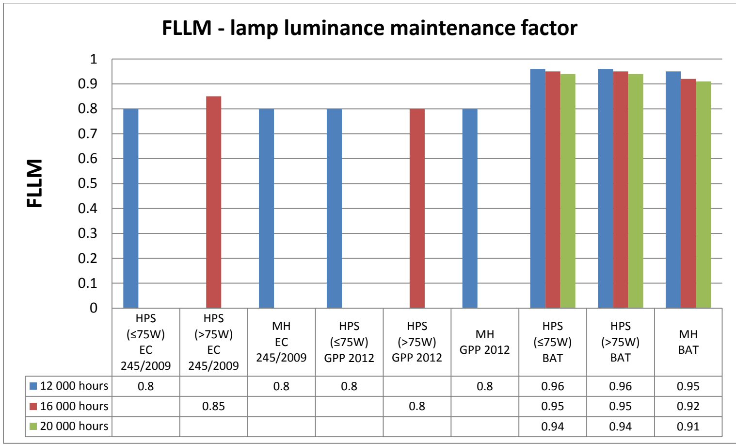
Figure 3-17 Lamp luminance maintenance factor for HPS and MH lamps according to the ecodesign regulation, the current GPP criteria and the best available technologies (BAT) 61,62
