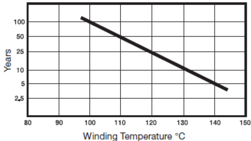
Figure 3-13 Typical trend of lifetime specification of magnetic control gear for HID lamps 50 with the winding temperature (°C)
