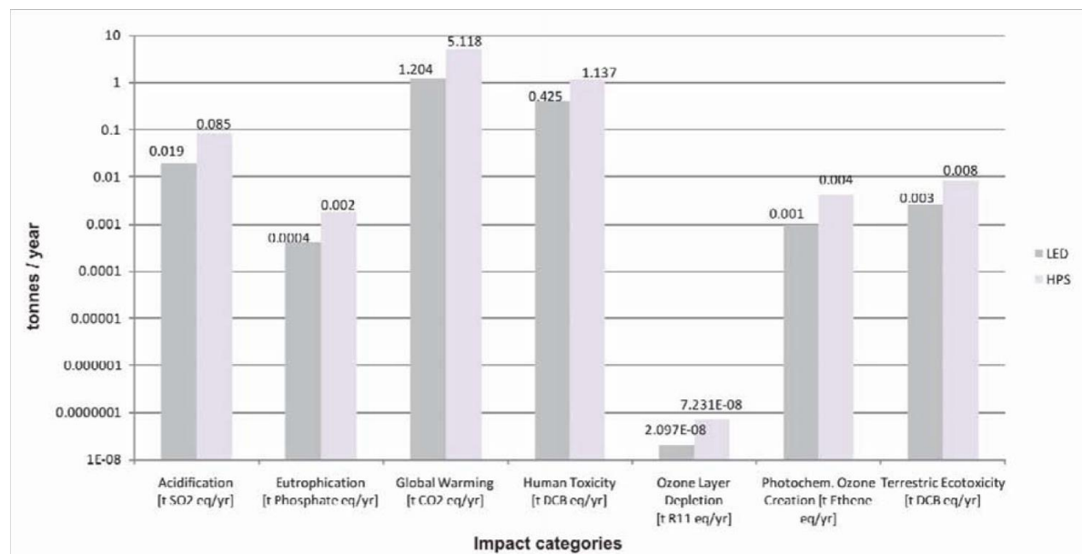
Figure 3-7 Overall environmental impacts of the LED and HPS technologies for public lighting (Lukman and Krajnc, 2011)
