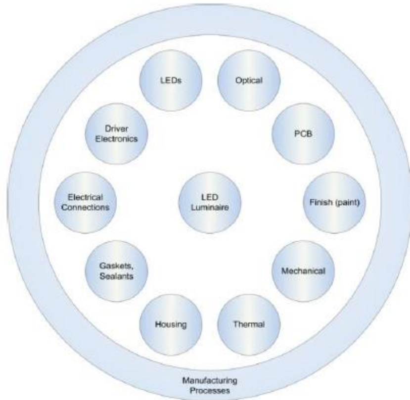
Figure 3-10 Total system or luminaire reliability is the product of all the individual reliability considerations: R_{luminaire} = R_{LEDs} * R_{optical} * R_{PCB} * R_{finish} * R_{mechanical} * R_{thermal} * R_{housing} * R_{gaskets/sealants} * R_{connections} * R_{driver} * R_{manufacturing} (taken from (LRSC, 2014))
