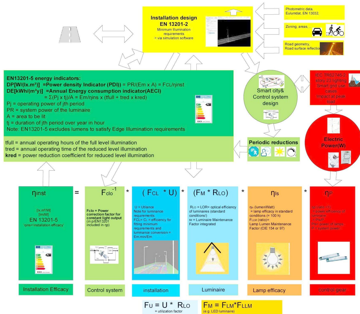
Figure 3-9 Components of a road lighting system and the most relevant performance parameters related to energy efficiency. The colour coding applied is: electrical efficiency (dark green), installation (dark blue), luminaire (sky blue), lamp (orange), control system (light green), control gear (red) and design process (yellow).
