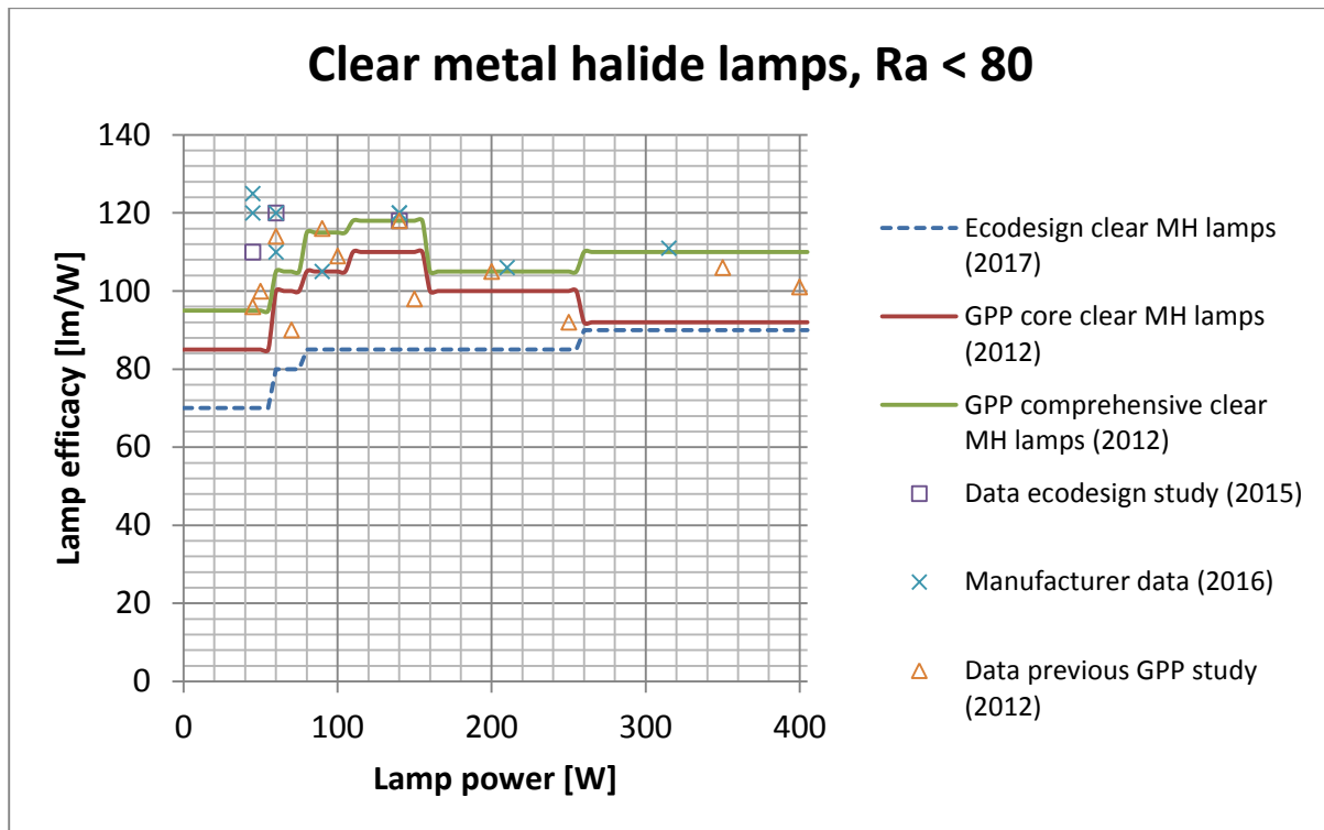
Figure 3-16 Lamp efficacy in function of lamp wattage for clear MH lamps with Ra < 80
