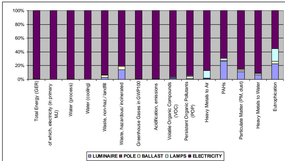
Figure 3-4 Life Cycle Impact (contribution of environmental impacts of lamps, ballast, luminaire and electricity use along their life cycle) (Van Tichelen et al., 2007)
