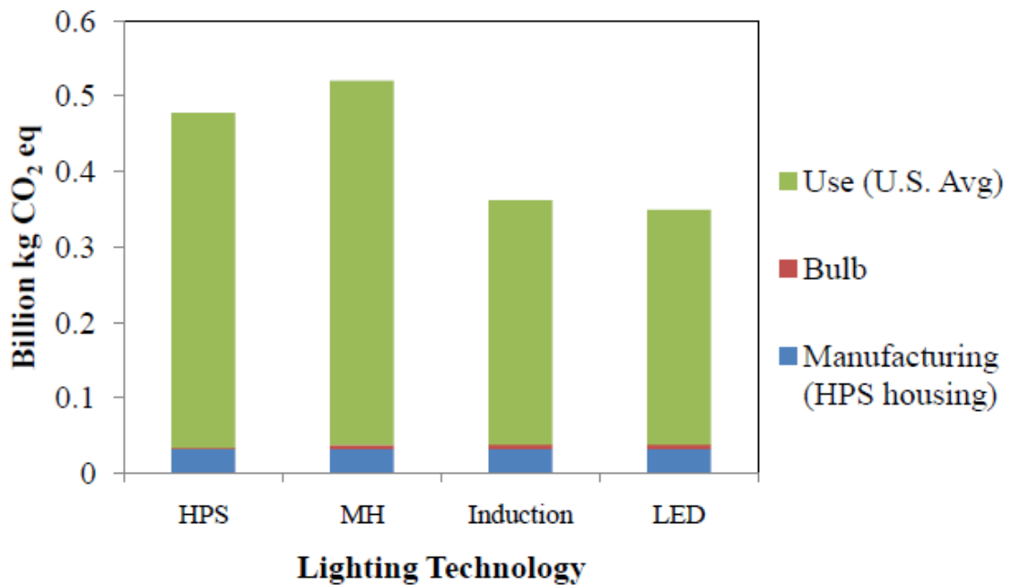
Figure 3-3 GWP emissions split for the manufacturing phase of bulb and housing and the use phase for different lamp technologies. The use phase was calculated with the US electricity mix (Hartley, D. et al. 2009)
