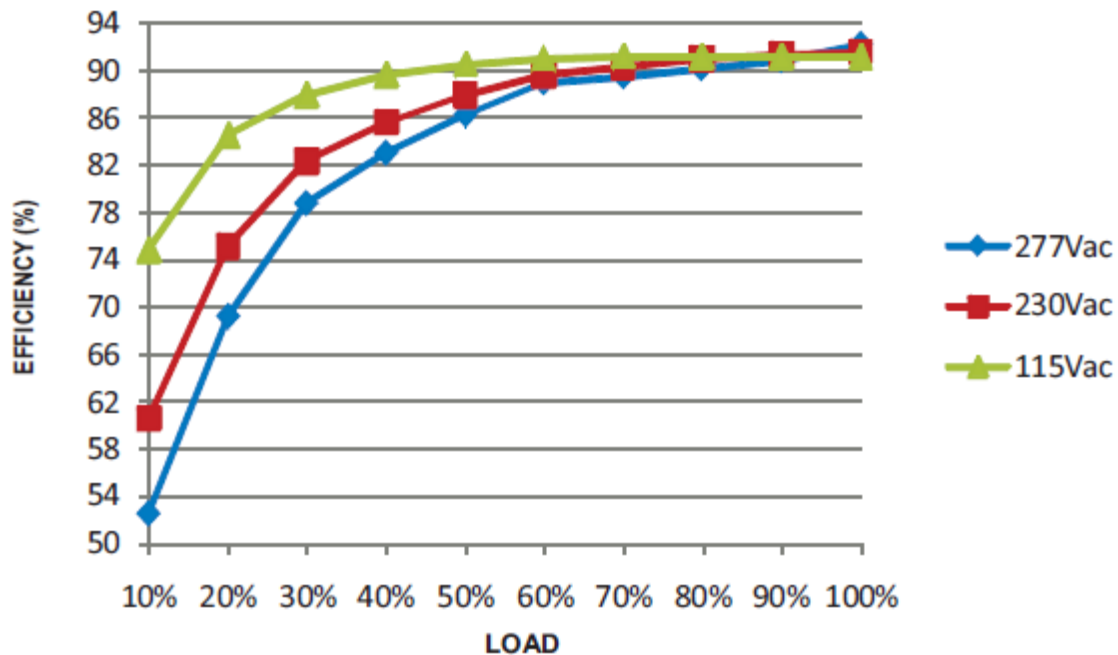
Figure 3-12 Efficiency vs. load for a LED driver (Mean Well, 2016)
