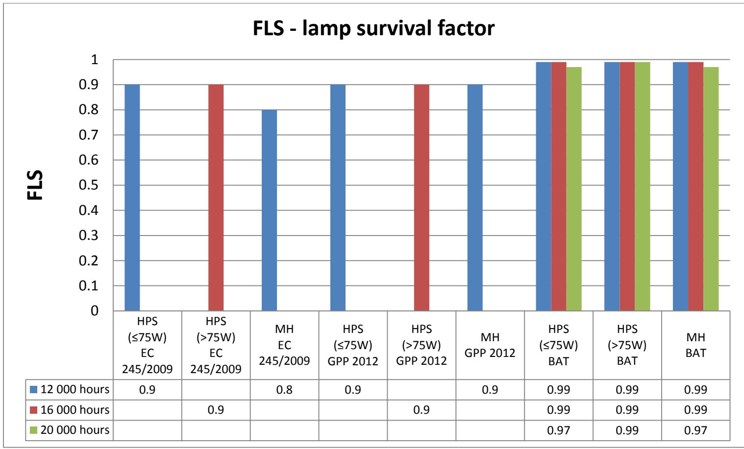
Figure 3-18 Lamp survival factor for HPS and MH lamps according to the ecodesign regulation, the current GPP criteria and the best available technologies (BAT)
