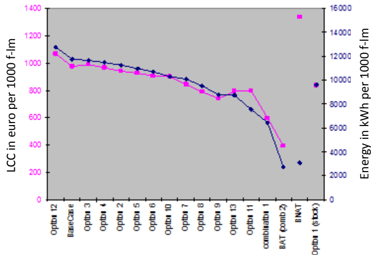
Figure 2-3 Different options ranked according to their 'energy saving potential' with LCC information for a reference slow traffic road (category S). The y-axis on the left side represents the life cycle costing in euro per 1000 useful lumen. The y-axis on the right represents the total energy consumption per 1000 useful lumen (1 lux on 1 m 2 ) (Van Tichelen et al., 2007)
