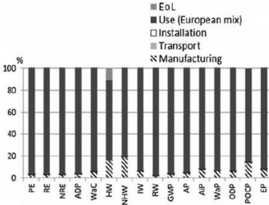
Figure 3-2 Division of environmental impacts of a LED downlight luminaire into life cycle stages with the energy consumption modelled with an average European electricity mix. Adapted from (Tähkämö, 2013).
