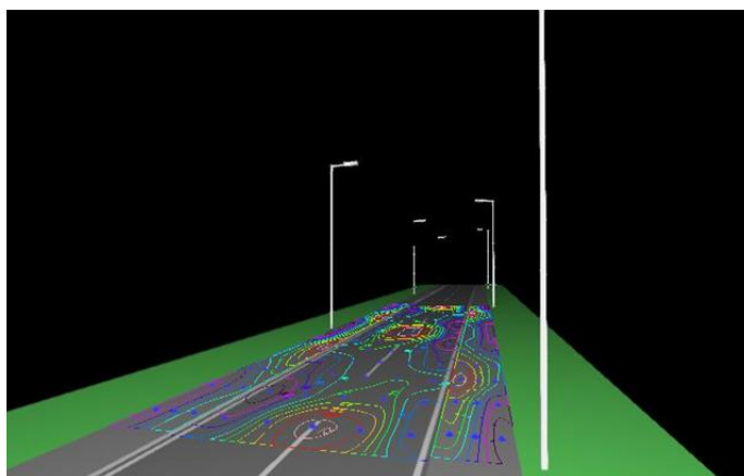
Figure 5-5 Utilance and other road lighting design parameters can be obtained from lighting design calculation software based on the photometric file of the luminaire 67
