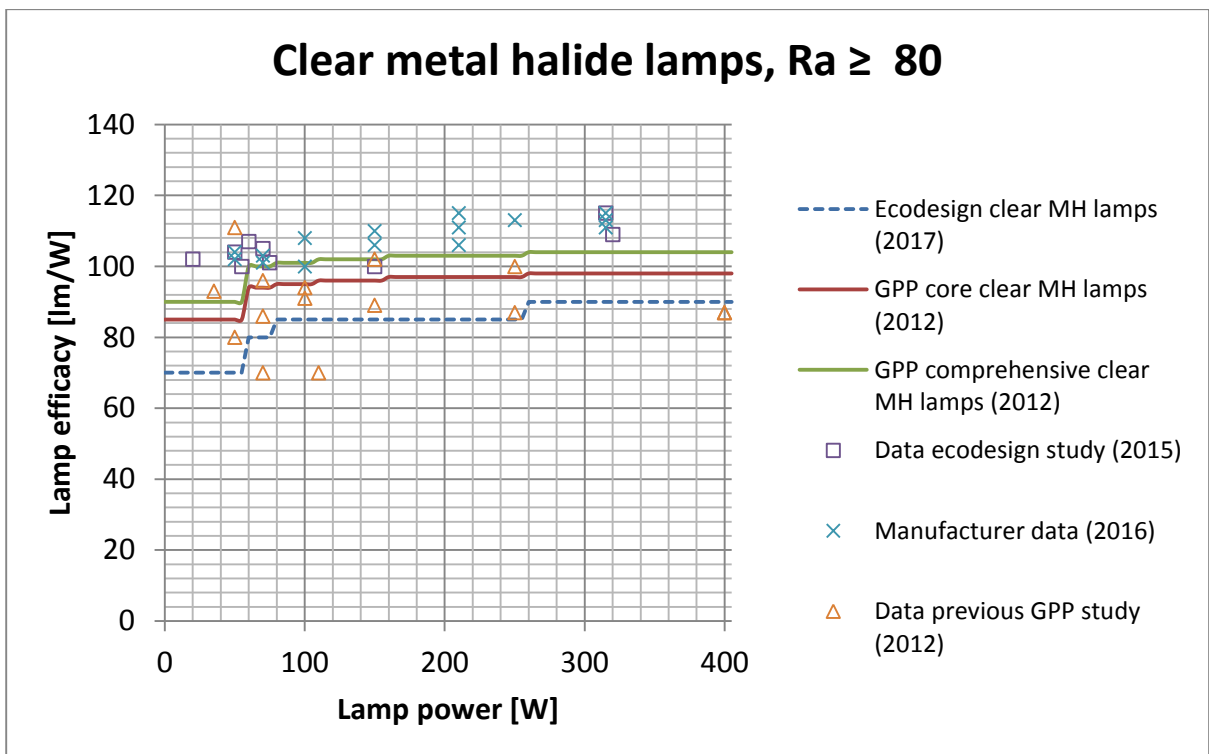
Figure 3-15 Lamp efficacy in function of lamp wattage for clear MH lamps with Ra ≥ 80
