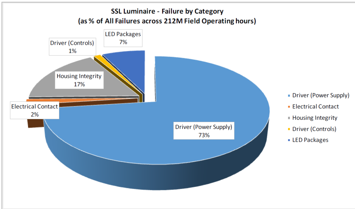
Figure 3-11 SSL luminaire failure modes, across 212 million field hours. Source: Appalachian Lighting Systems, Inc. (taken from LRSC (2014))
