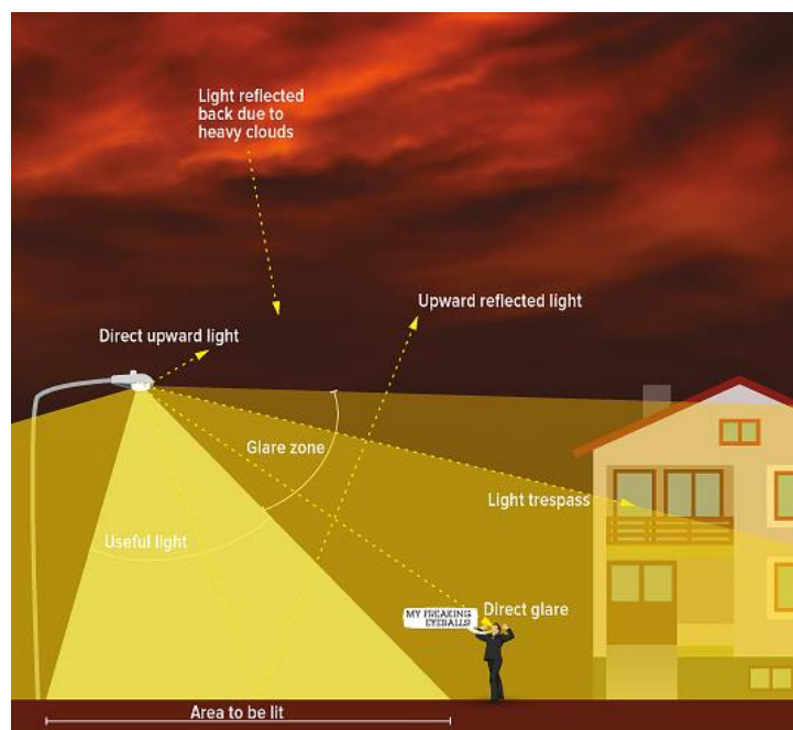
Figure 3-8 The info-graphic above illustrates the different components of light pollution and what “good” lighting looks like. (Image credit: Anezka Gocova, taken from https://astronomynow.com/2015/04/11/international-dark-sky-week-2015/ )
