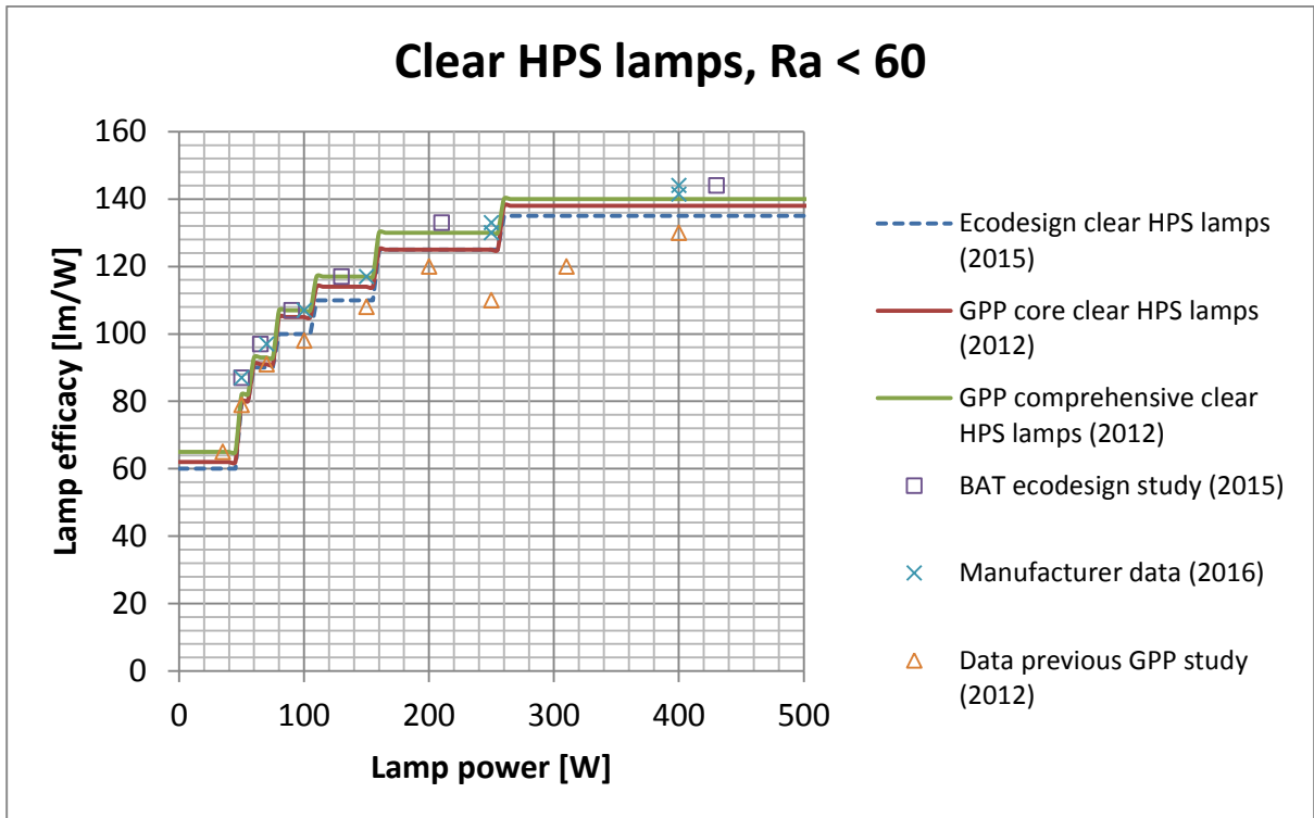
Figure 3-14 Lamp efficacy in function of lamp wattage for clear HPS lamps with Ra < 60
