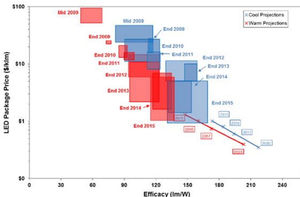
Figure 2-2 Price-Efficacy tradeoff for LED Packages at 1 W/mm 2 (equiv. 35 A/cm 2 ) and 25°C (DOE, 2016)
